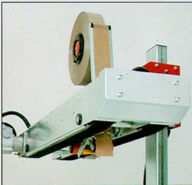
Double drive belts
