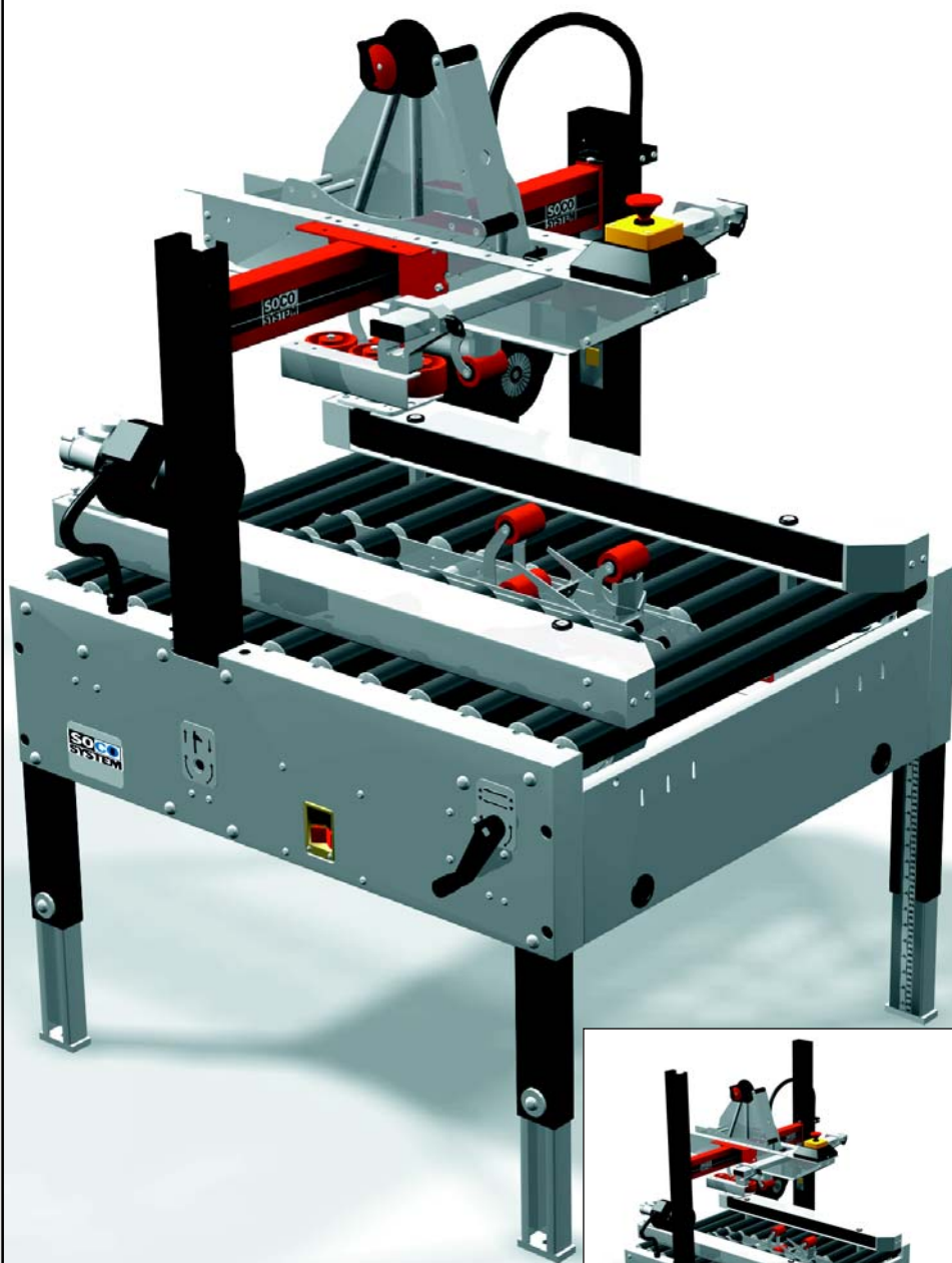
Crank Handle adjustment for carton size
