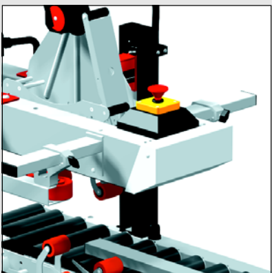
Manual side pressure guides and centrally placed emergency stop
